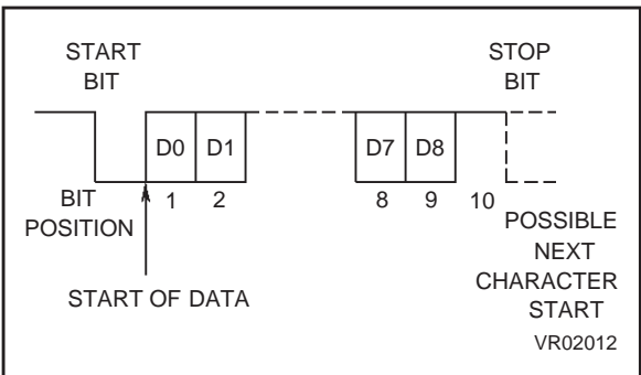
Figure 27. Character Format
