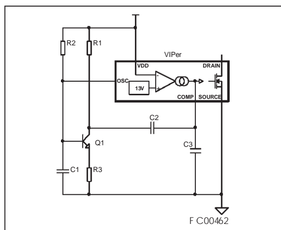
Figure 16: Slope Compensation
