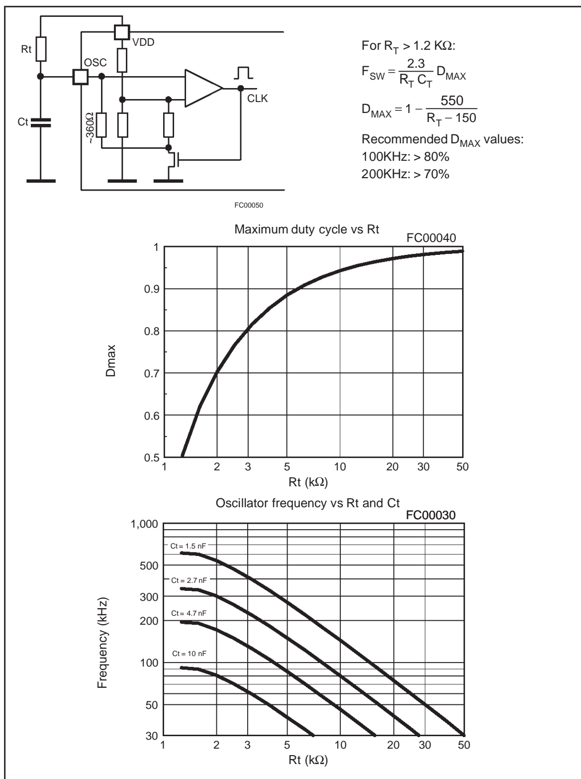
Figure 7: Oscillator
