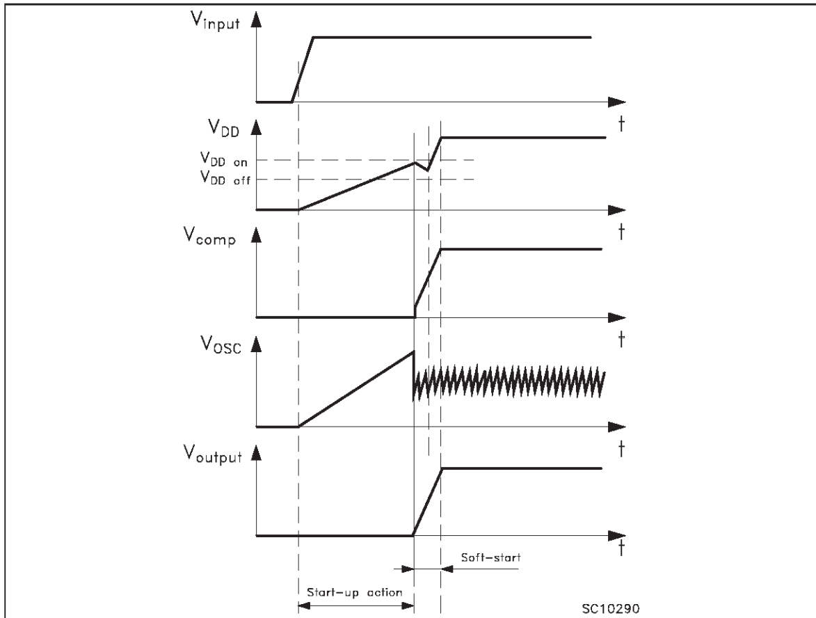
Figure 5: Start-up Waveforms
