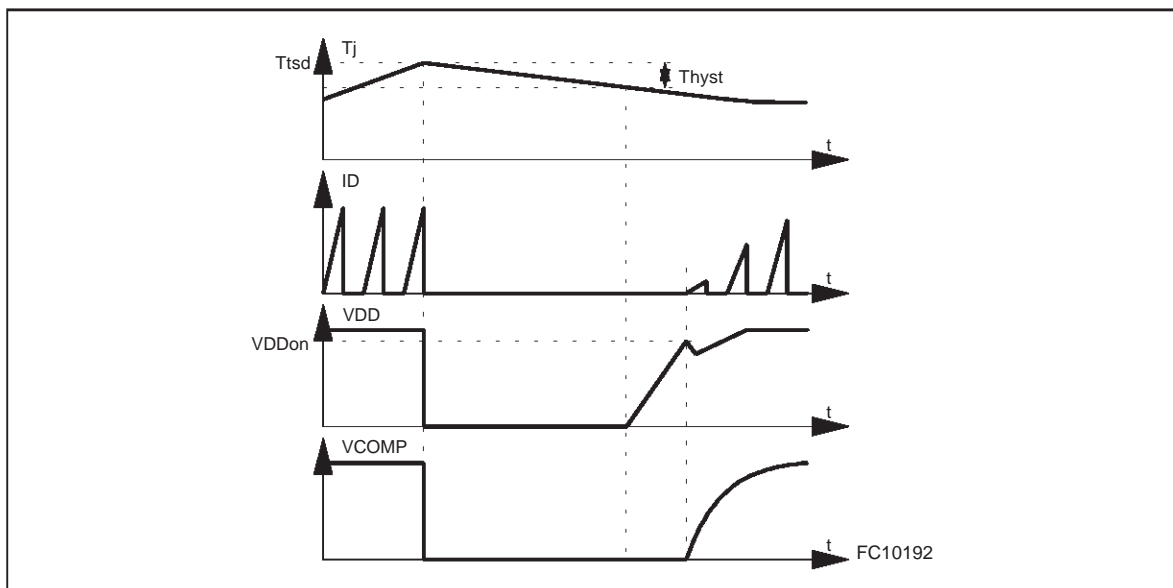
Figure 6: Overtemperature Protection
