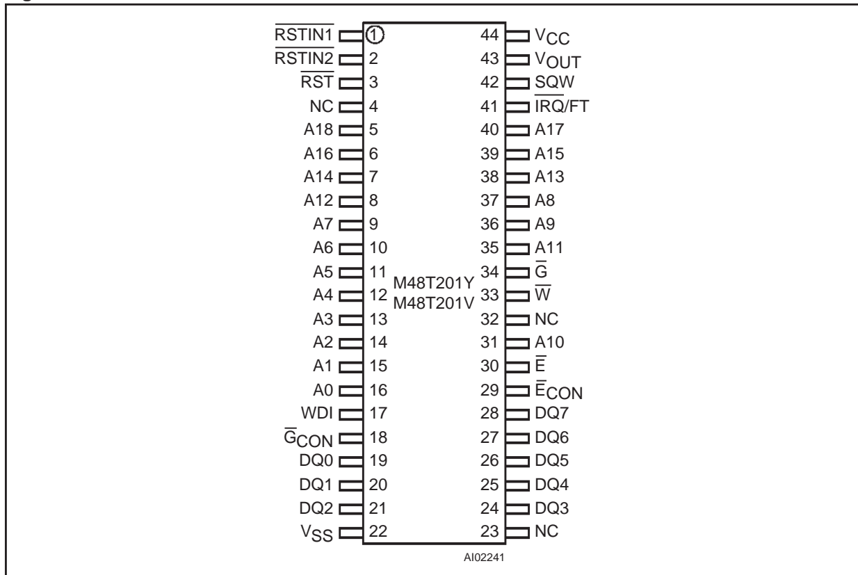
Figure 3. SOIC Connections
