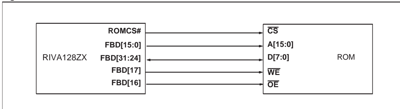
Figure 63. ROM interface
