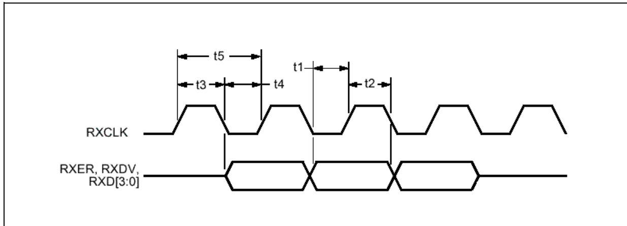
Figure 5. MII Receive Timing
