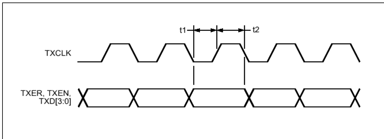
Figure 6. MII Transmit Timing
