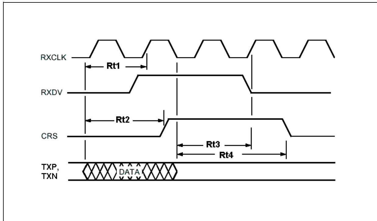
Figure 7. Receive Timing
