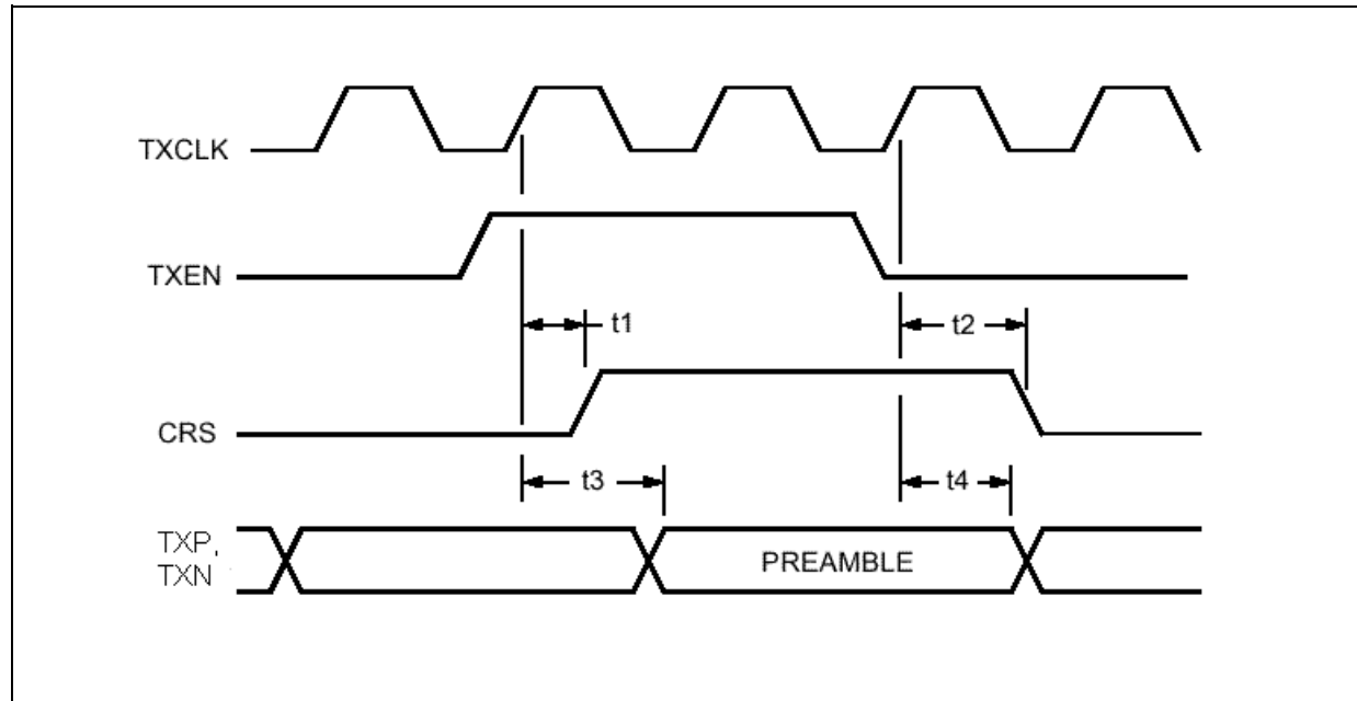
Figure 8. Transmit Timing
