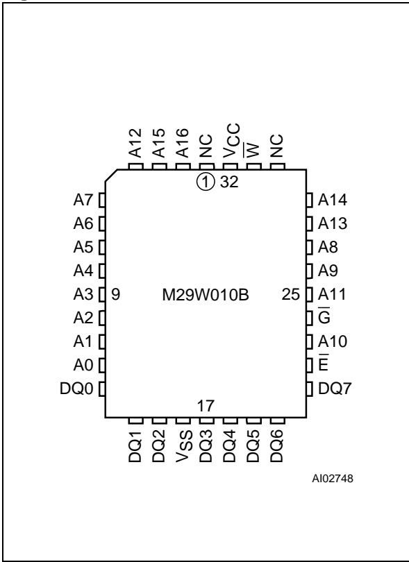
Figure 2. PLCC Connections
