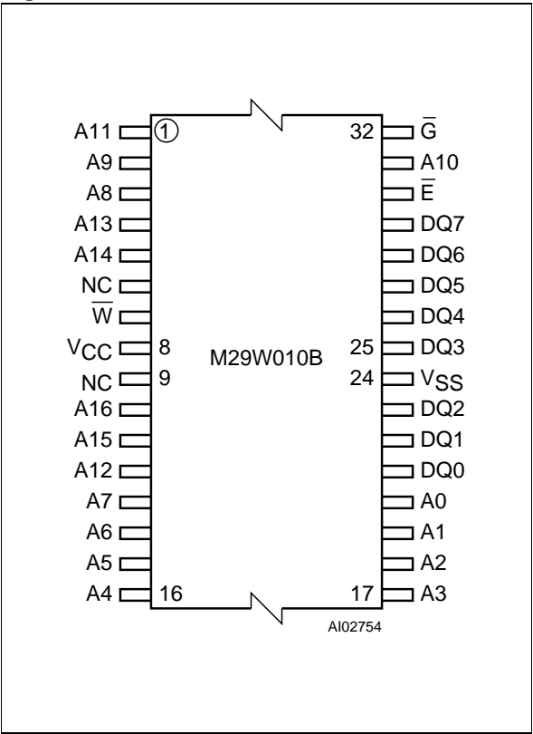
Figure 3. TSOP Connections
