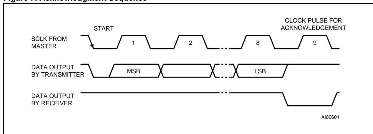
Figure 7. Acknowledgment Sequence
