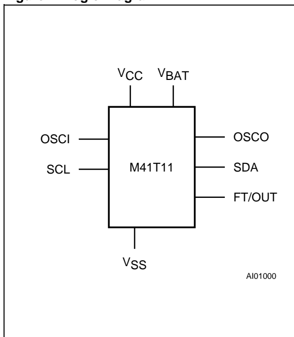
Figure 1. Logic Diagram
