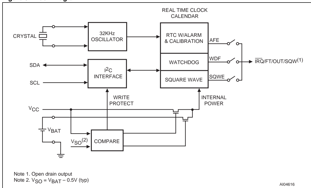
Figure 8. Block Diagram
