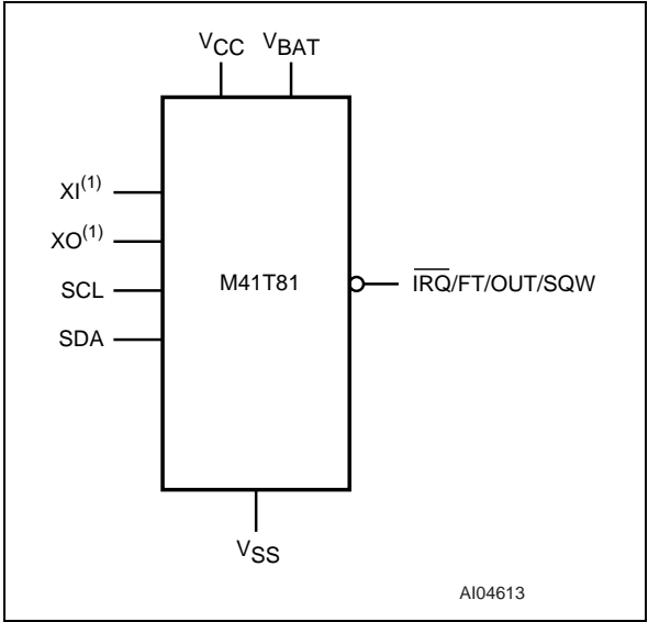
Figure 4. Logic Diagram
