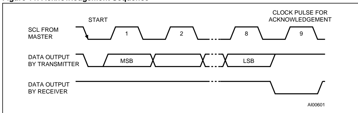
Figure 11. Acknowledgement Sequence
