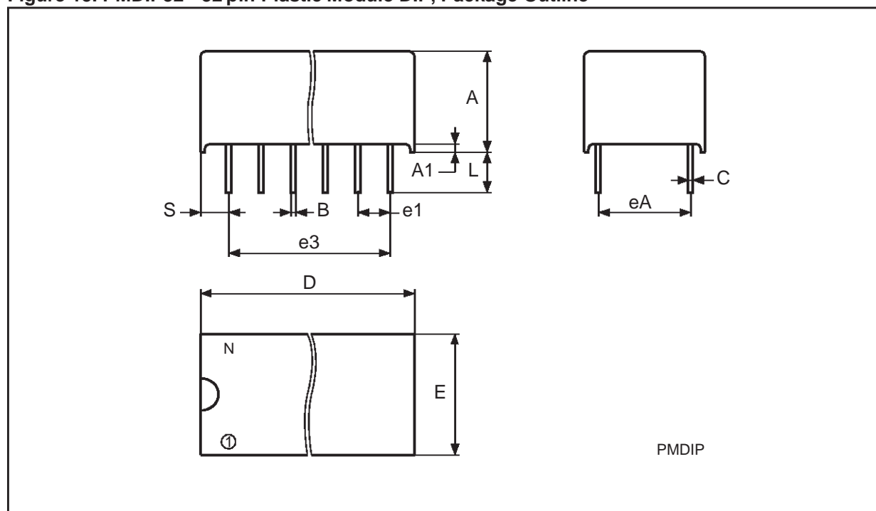
Figure 15. PMDIP32 - 32 pin Plastic Module DIP, Package Outline
