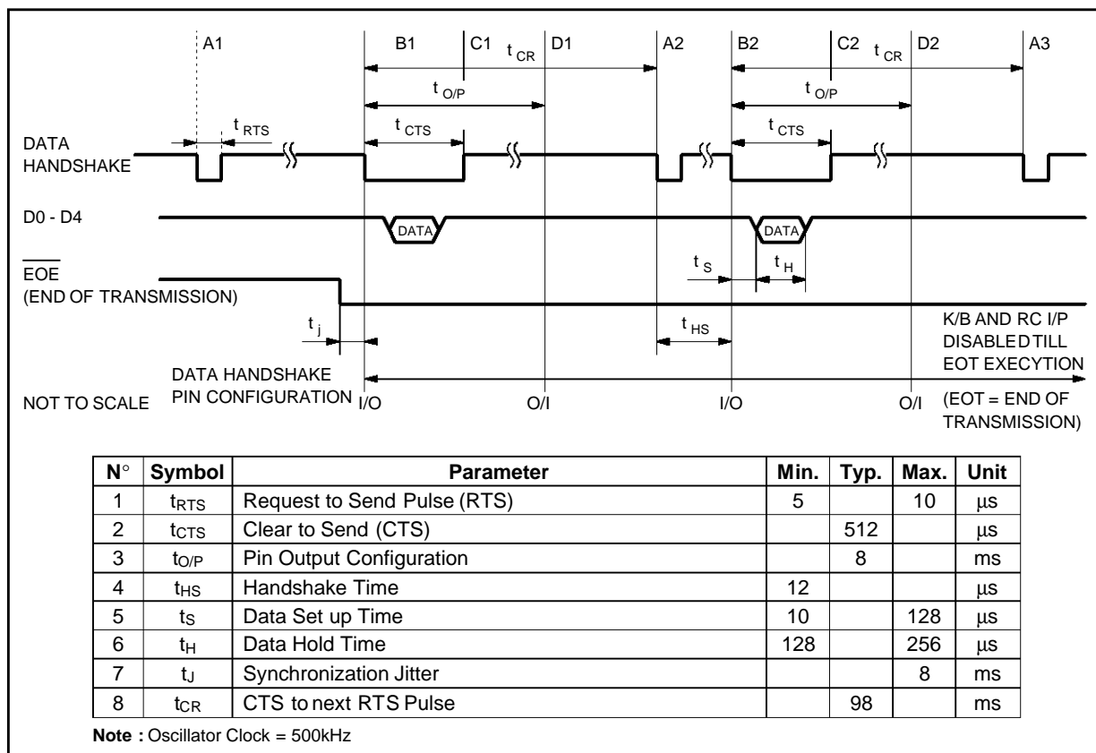
Figure 6 : Data-input-timing
