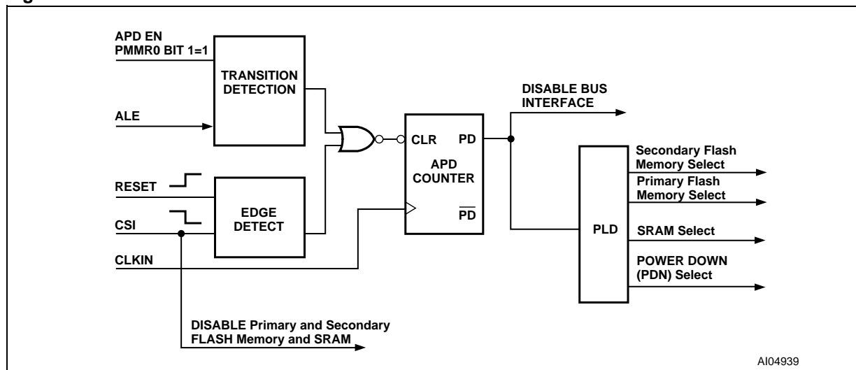
Figure 32. APD Unit
