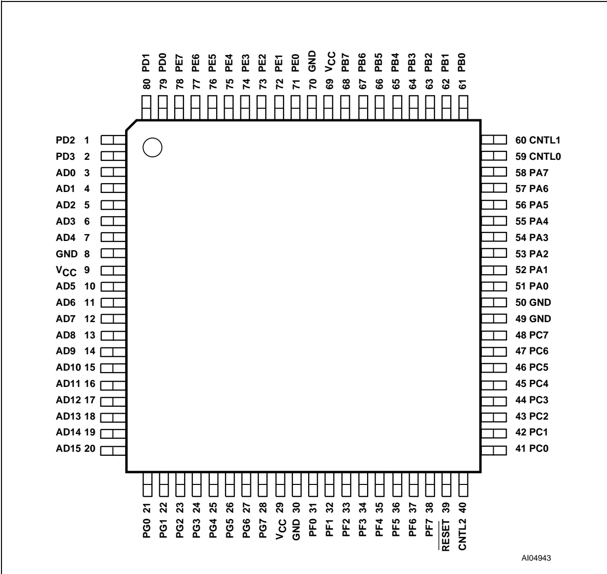
Figure 3. TQFP Connections
