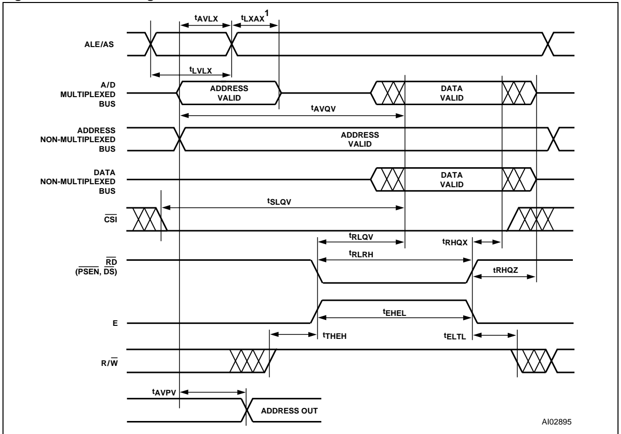
Figure 42. READ Timing
