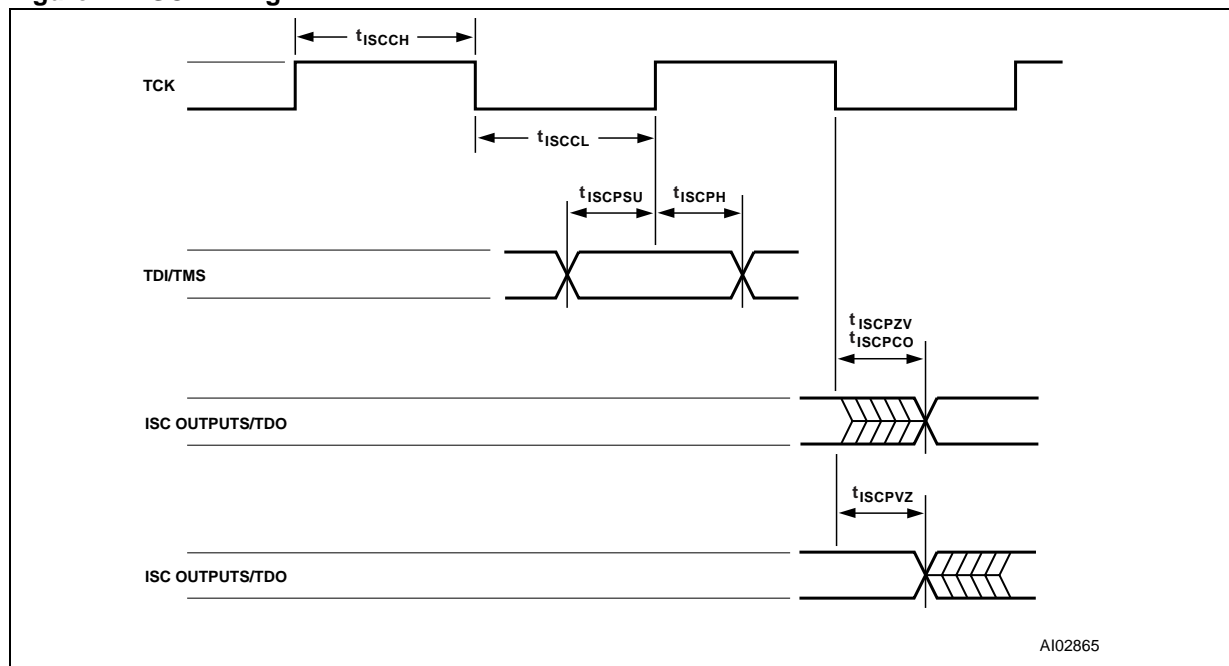
Figure 47. ISC Timing
