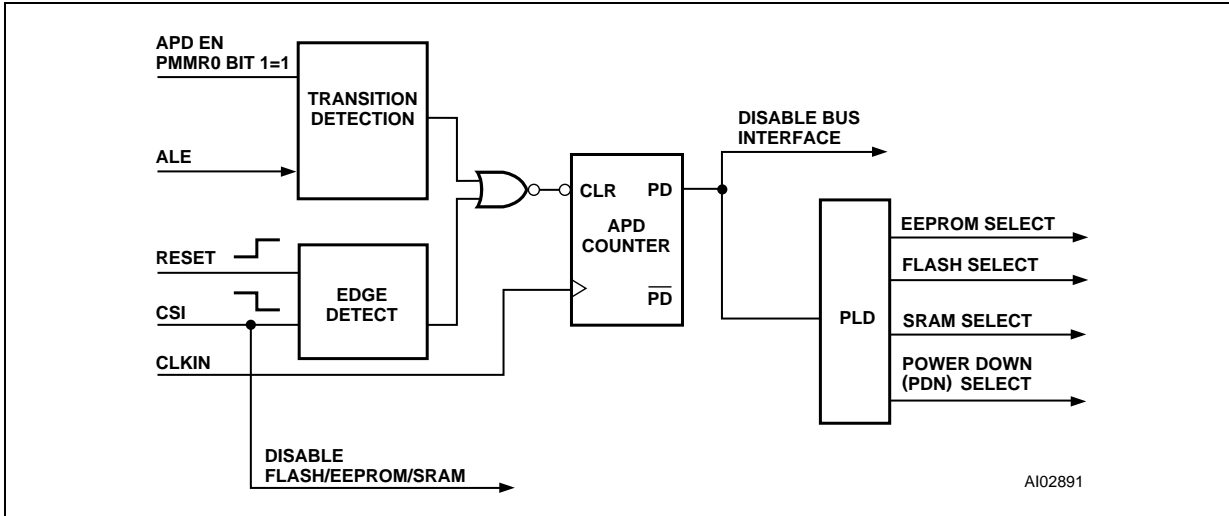
Figure 29. APD Unit
