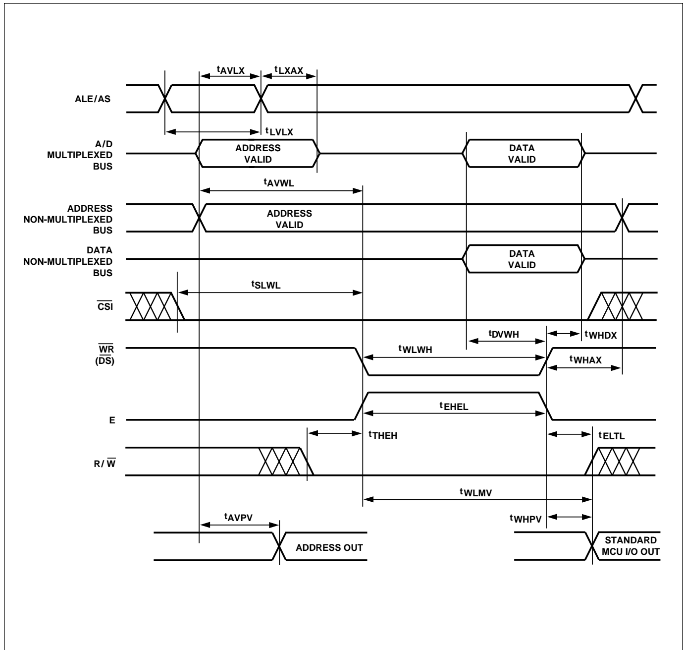
Figure 34. Write Timing
