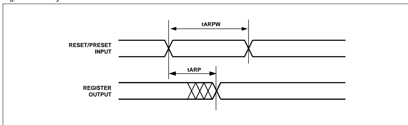
Figure 42. Asynchronous Reset/Preset
