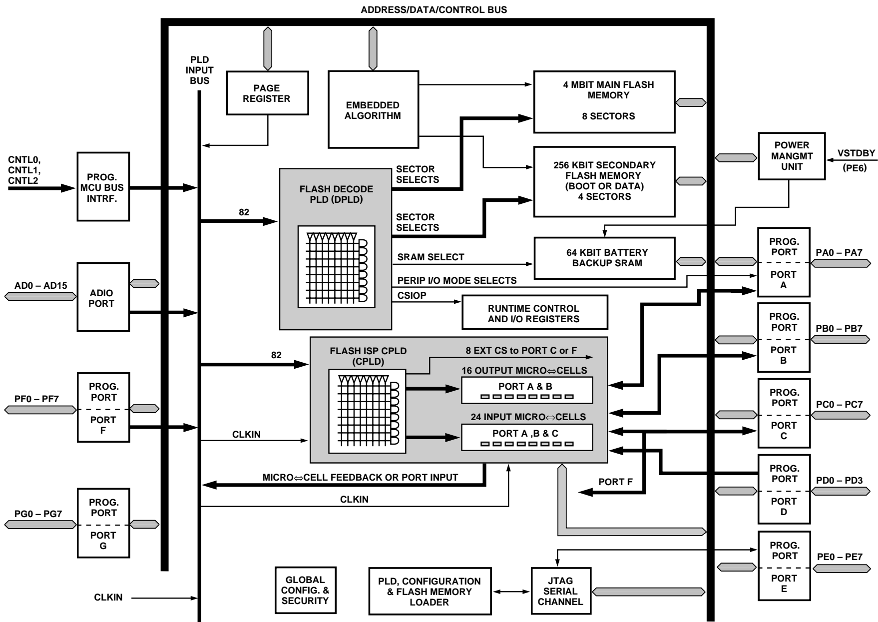
Figure 1. PSD835G2 Block Diagram
