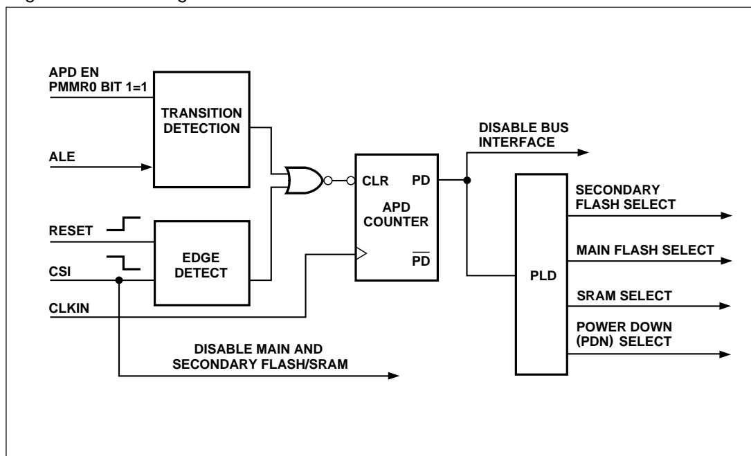
Figure 29. APD Logic Block
