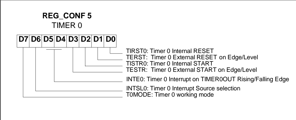
Figure 10.5 Configuration Register 5
