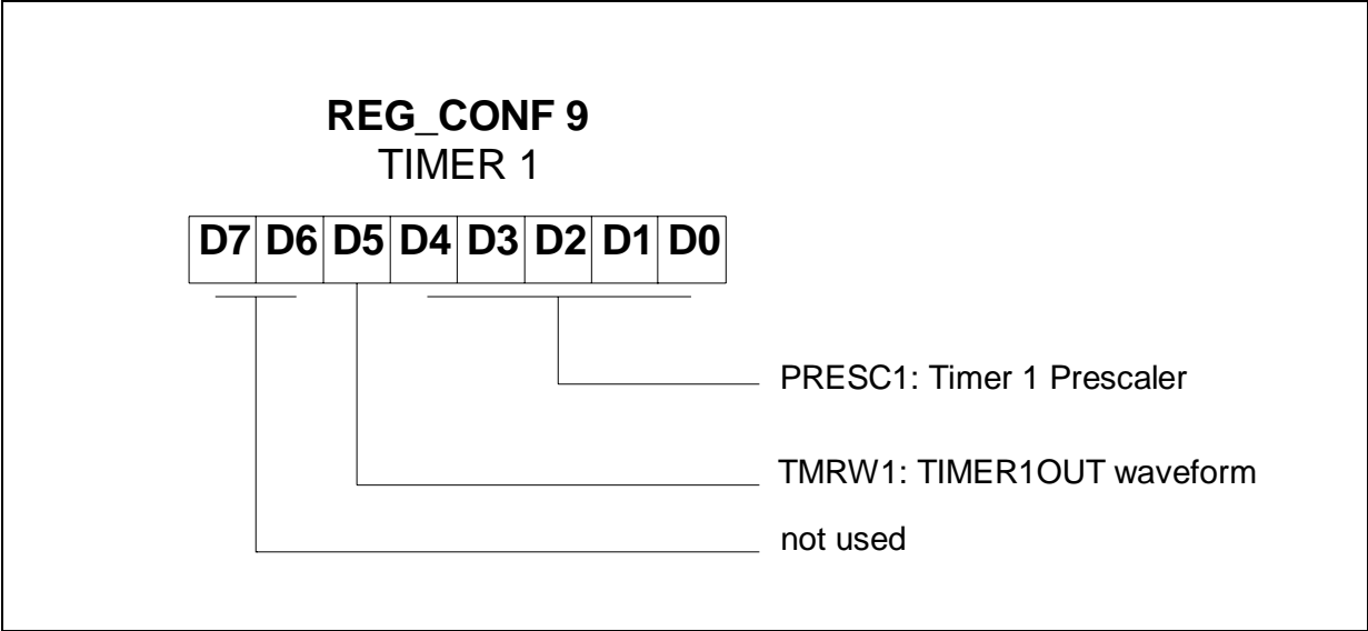
Figure 10.9 Configuration Register 9
