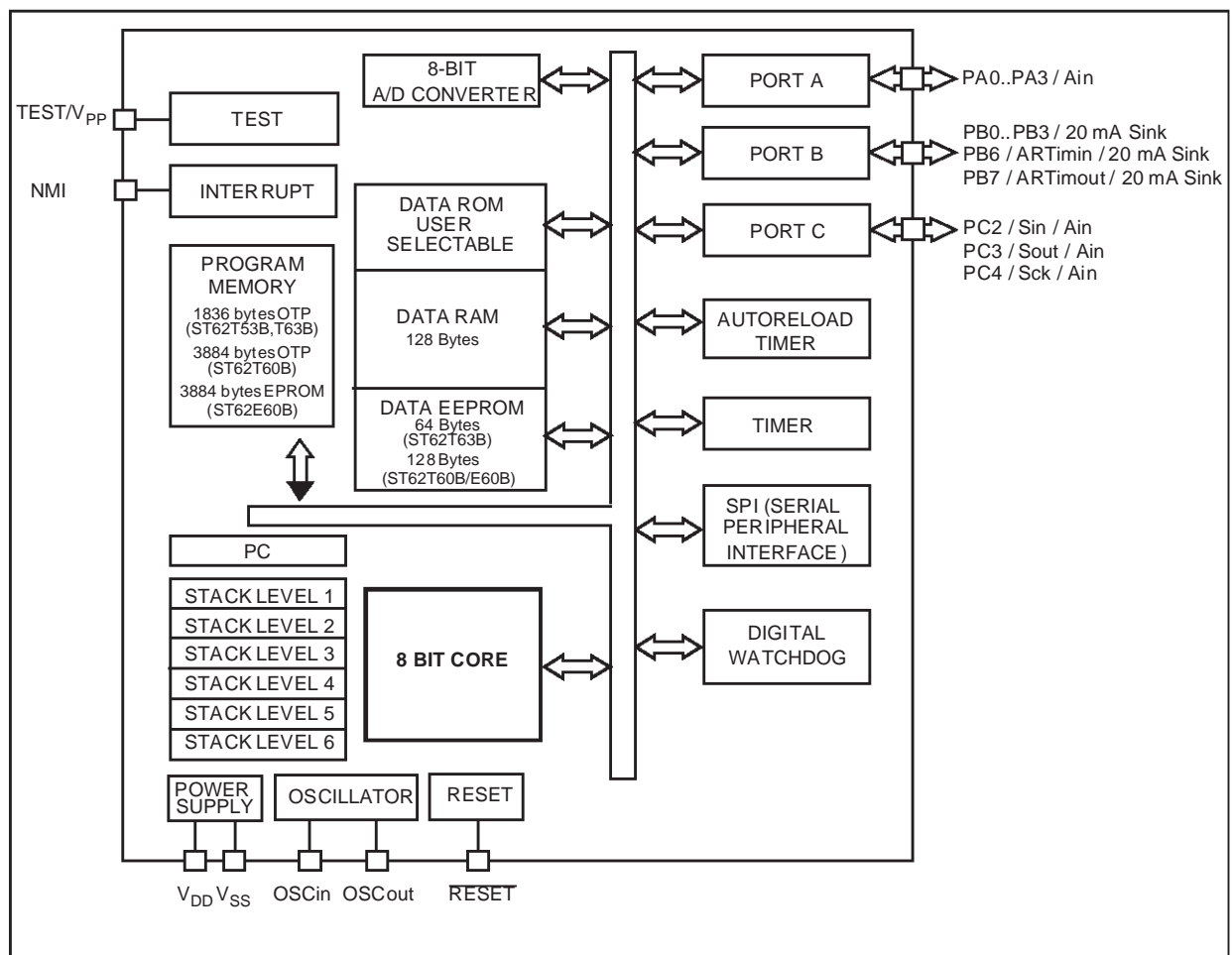
Figure 1. Block Diagram
