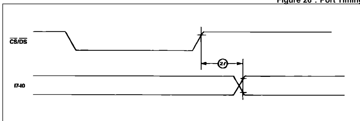
Figure 26 : Port Timing
