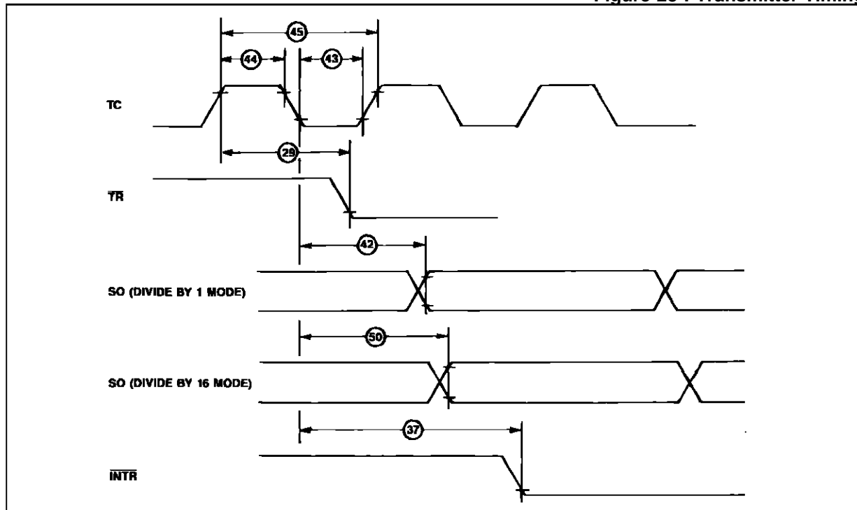
Figure 28 : Transmitter Timing
