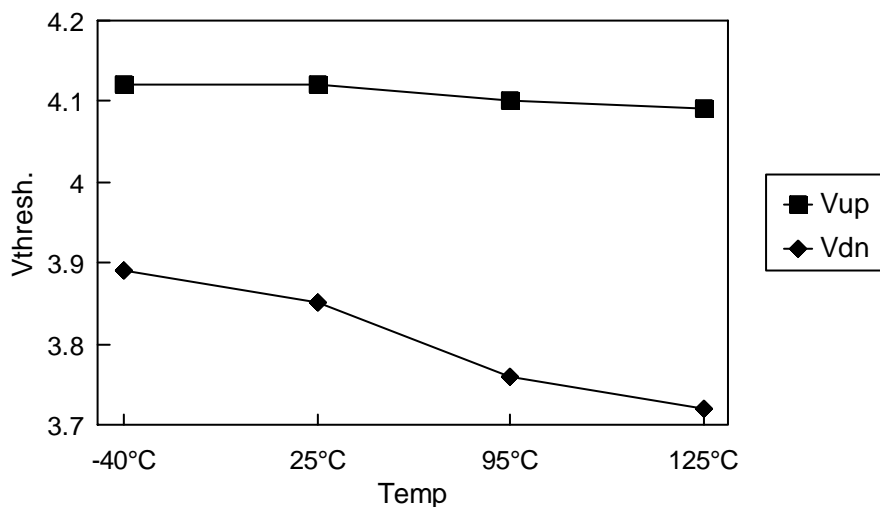
Figure 47. LVD thresholds versus temperature
