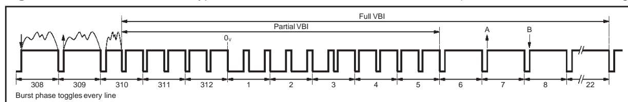
Figure 3 : PAL-BDGIH, PAL-N Typical VBI Waveform, Non-interlaced Mode ("CCIR-like" Line Numbering)
