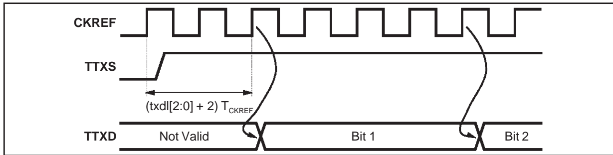
Figure 26 : "TTXS Rising" to "First Valid Sample" Delay for \text{txdl}[2:0] = 0
