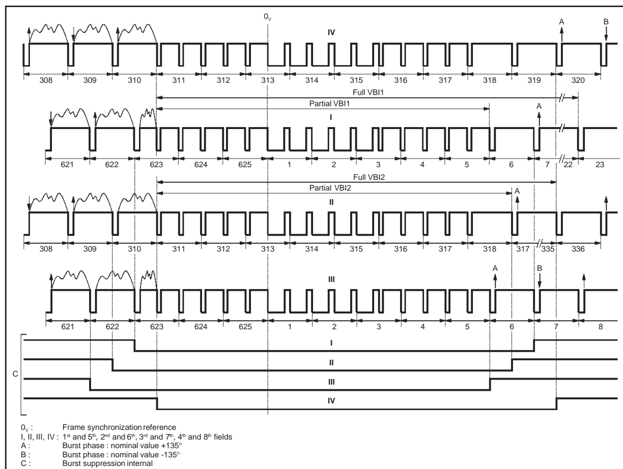
Figure 3 : PAL-BDGIH, PAL-N Typical VBI Waveform, Non-interlaced Mode ("CCIR-like" Line Numbering)
