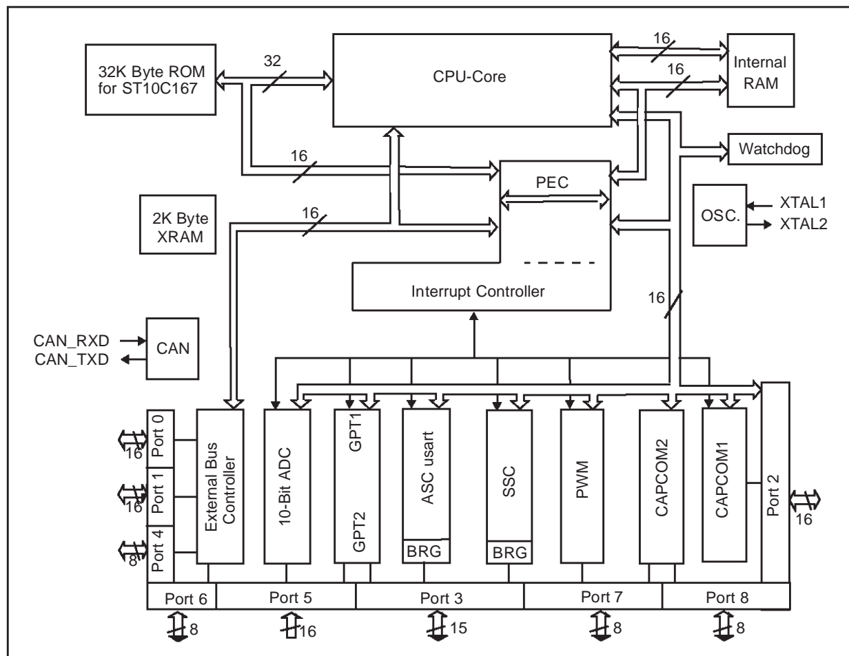
Figure 3 : Block diagram
