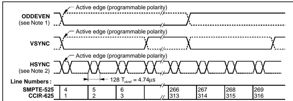
Figure 9 : ODDEV, VSYNC and HSYNC Waveforms
