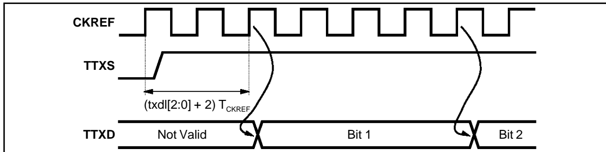
Figure 26 : “TTXS Rising” to “First Valid Sample” Delay for \text{txdl}[2:0] = 0
