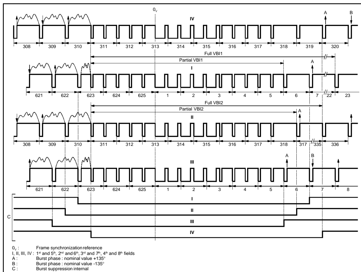
Figure 3 : PAL-BDGI, PAL-N Typical VBI Waveform, Non-interlaced Mode ("CCIR-like" Line Numbering)
