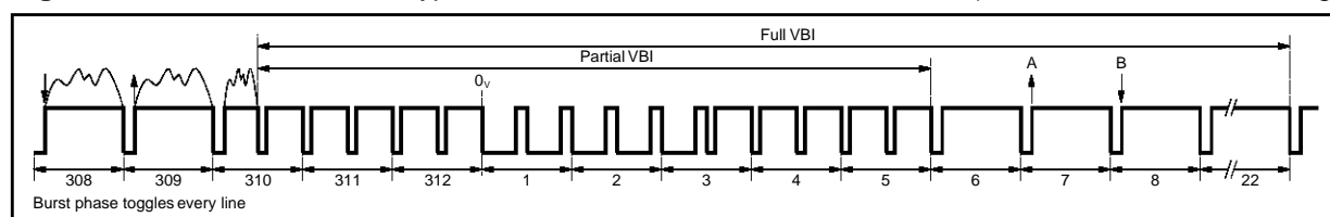
Figure 3 : PAL-BDGI, PAL-N Typical VBI Waveform, Non-interlaced Mode ("CCIR-like" Line Numbering)
