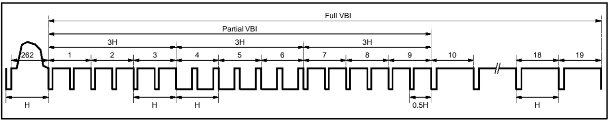
Figure 5 : NTSC-M Typical VBI Waveforms, Non-interlaced Mode ("SMPTE-like" Line Numbering)
