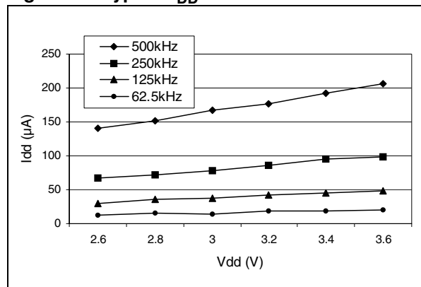
Figure 58. Typical I_{DD} SLOW mode
