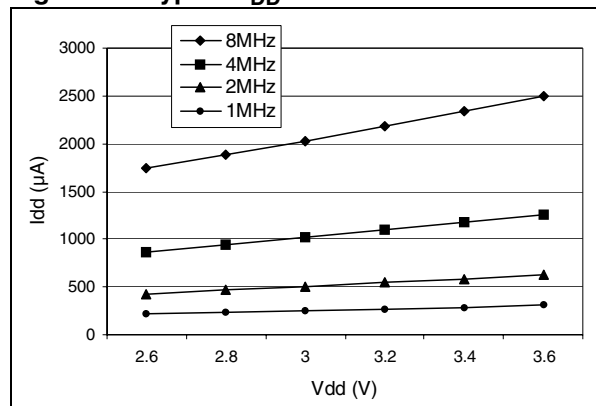
Figure 57. Typical I_{DD} in RUN mode
