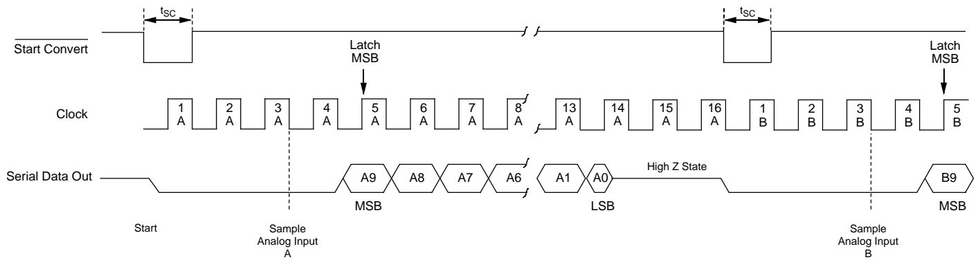
Figure 6 - Free Run Mode Timing Diagram
