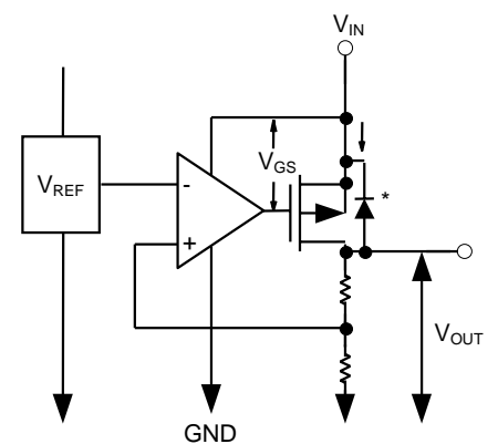
Figure 5 Error amplifier
