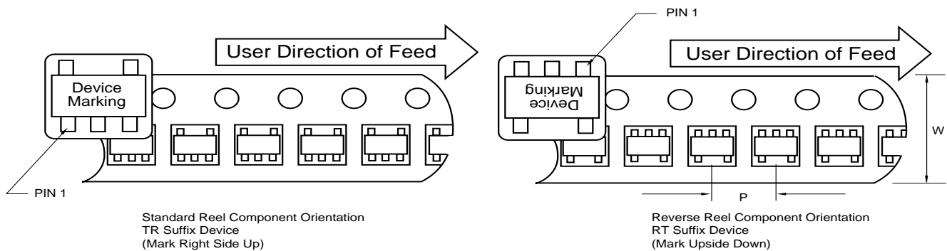
Carrier Tape, Number of Components Per Reel and Reel Size
