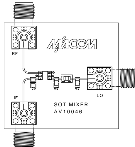
MIXER PCB
