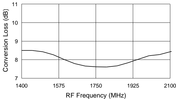
CONVERSION LOSS vs. FREQUENCY
