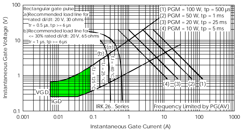
Fig. 12- Gate Characteristics
