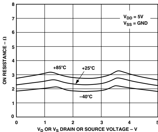
Figure 5. On Resistance as a Function of V_D ( V_S ) for Different Temperatures; V_{DD} = 5\text{ V}
