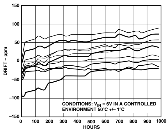
TPC 25. ADR381 Long-Term Drift
