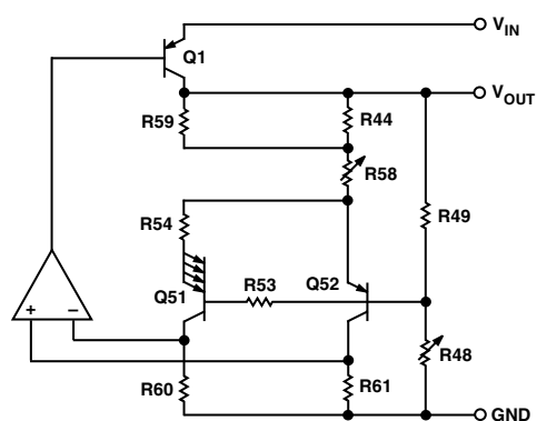
Figure 1. Simplified Schematic
