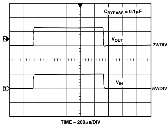
TPC 22. ADR381 Turn-On/Turn-Off Response at 5 V
