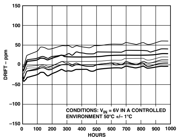
TPC 24. ADR380 Long-Term Drift
