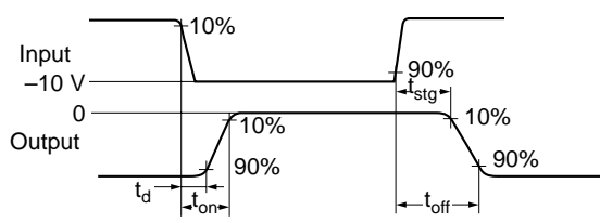
Response Waveform
