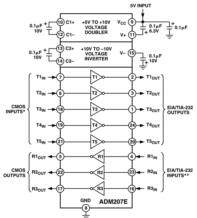
Figure 3. ADM207E Pin Configuration
