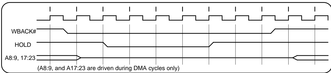
Figure 6.1 WBACK# Timing
