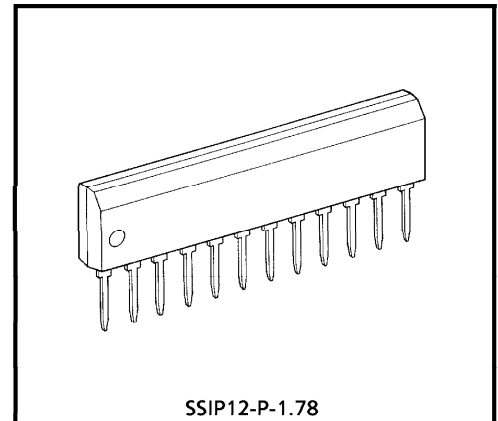
SSIP12-P-1.78 Weight : 0.65g (Typ.)
