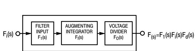
Figure 4. Loop Filter Block Diagram
