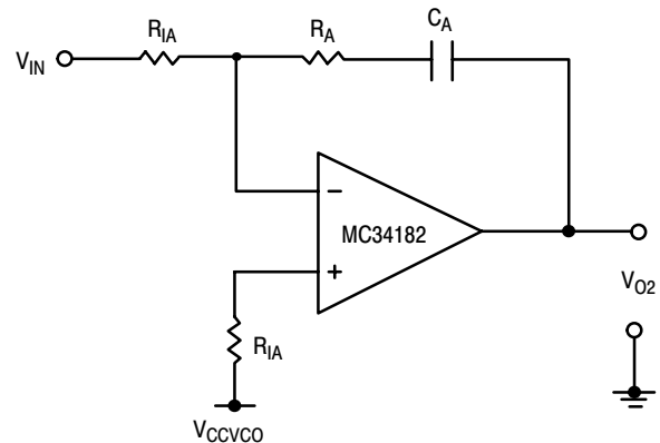
Figure 7. Integrator Subsection
