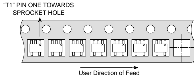
Figure 10. DFT1 (SC88A) Reel Configuration/Orientation
