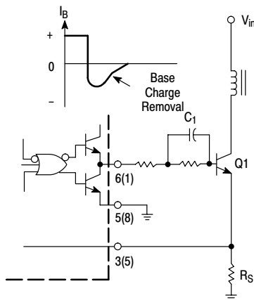
Figure 29. Bipolar Transistor Drive
