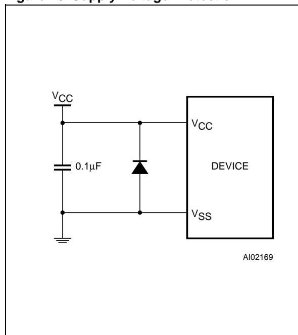
Figure 16. Supply Voltage Protection
