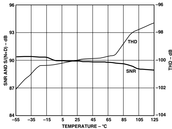
TPC 6. SNR, THD vs. Temperature
