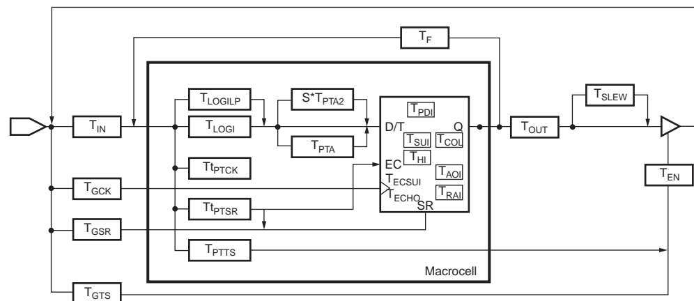
Figure 1: XC9500XV Detailed Timing Model
