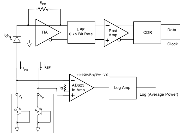
Figure 14. Conceptual Incoming Optical Power Monitoring Circuit.
