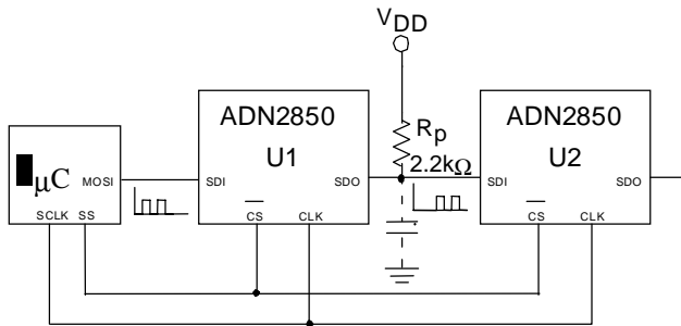
Figure 5. Daisy Chain Configuration
