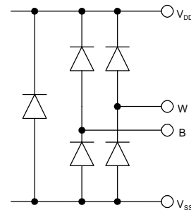
Figure 8. Maximum Terminal Voltages Set by V_{DD} & V_{SS}
