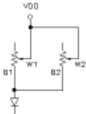
Figure 15. Reduce Resistance by half with linear adjustment characteristics
