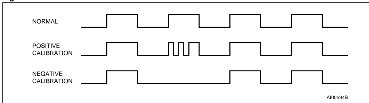
Figure 11. Clock Calibration
