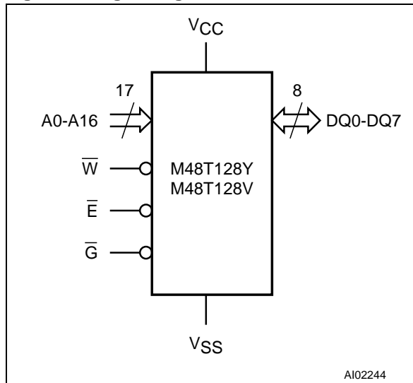
Figure 2. Logic Diagram
