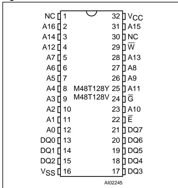
Figure 3. DIP Connections
