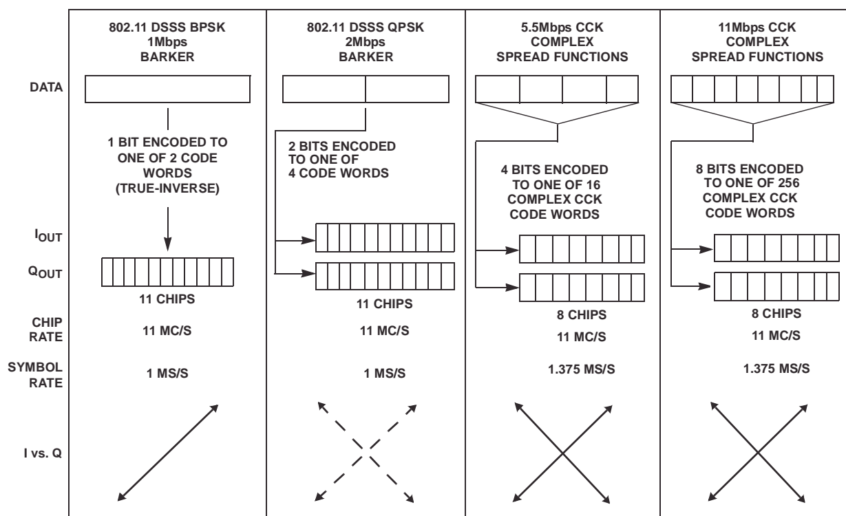
FIGURE 13. MODULATION MODES
