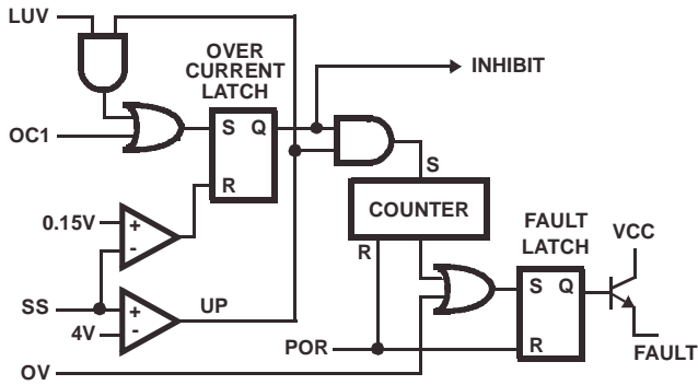
FIGURE 4. FAULT LOGIC - SIMPLIFIED SCHEMATIC
