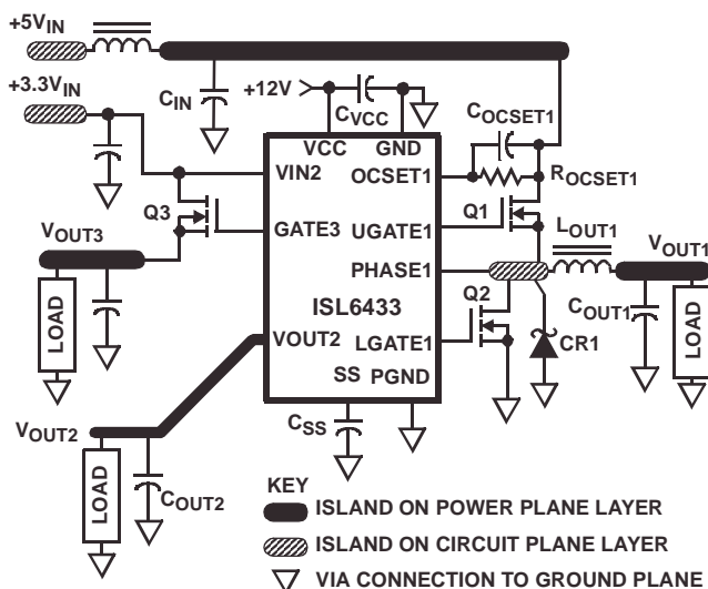
FIGURE 7. PRINTED CIRCUIT BOARD POWER PLANES AND ISLANDS
