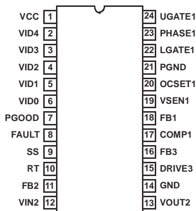
ISL6433 (SOIC) TOP VIEW
