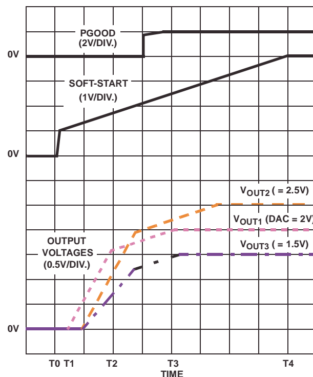
FIGURE 3. SOFT-START INTERVAL
