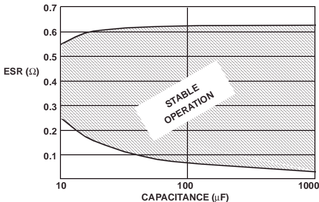
FIGURE 10. C OUT2 OUTPUT CAPACITOR
