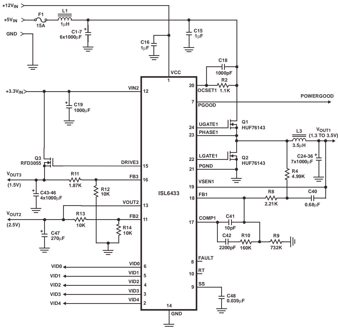
FIGURE 12. APPLICATION CIRCUIT
