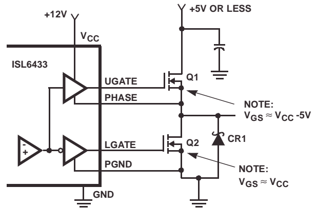
FIGURE 11. OUTPUT GATE DRIVERS
