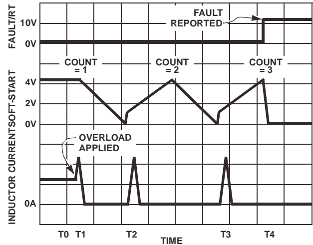
FIGURE 5. OVERCURRENT OPERATION
