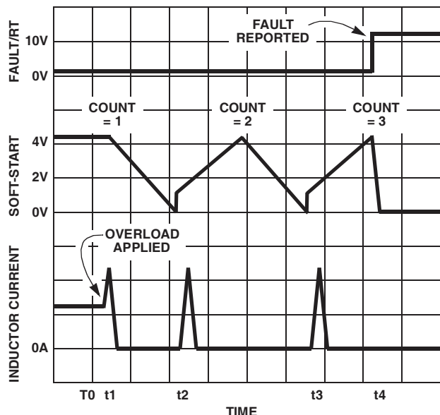
FIGURE 5. OVERCURRENT OPERATION
