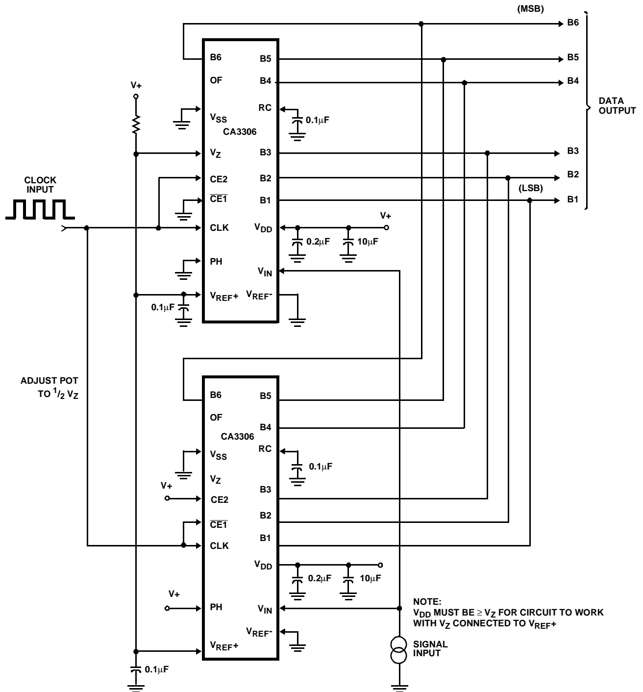
FIGURE 18. TYPICAL CA3306 6-BIT RESOLUTION CONFIGURATION WITH DOUBLE SAMPLING RATE CAPABILITY
