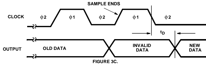
FIGURE 3. PULSE MODE
