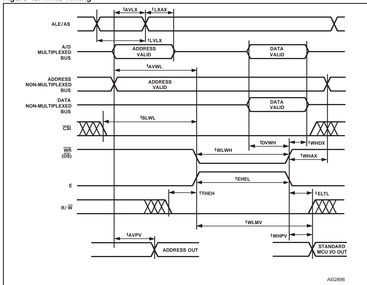
Figure 42. Write Timing
