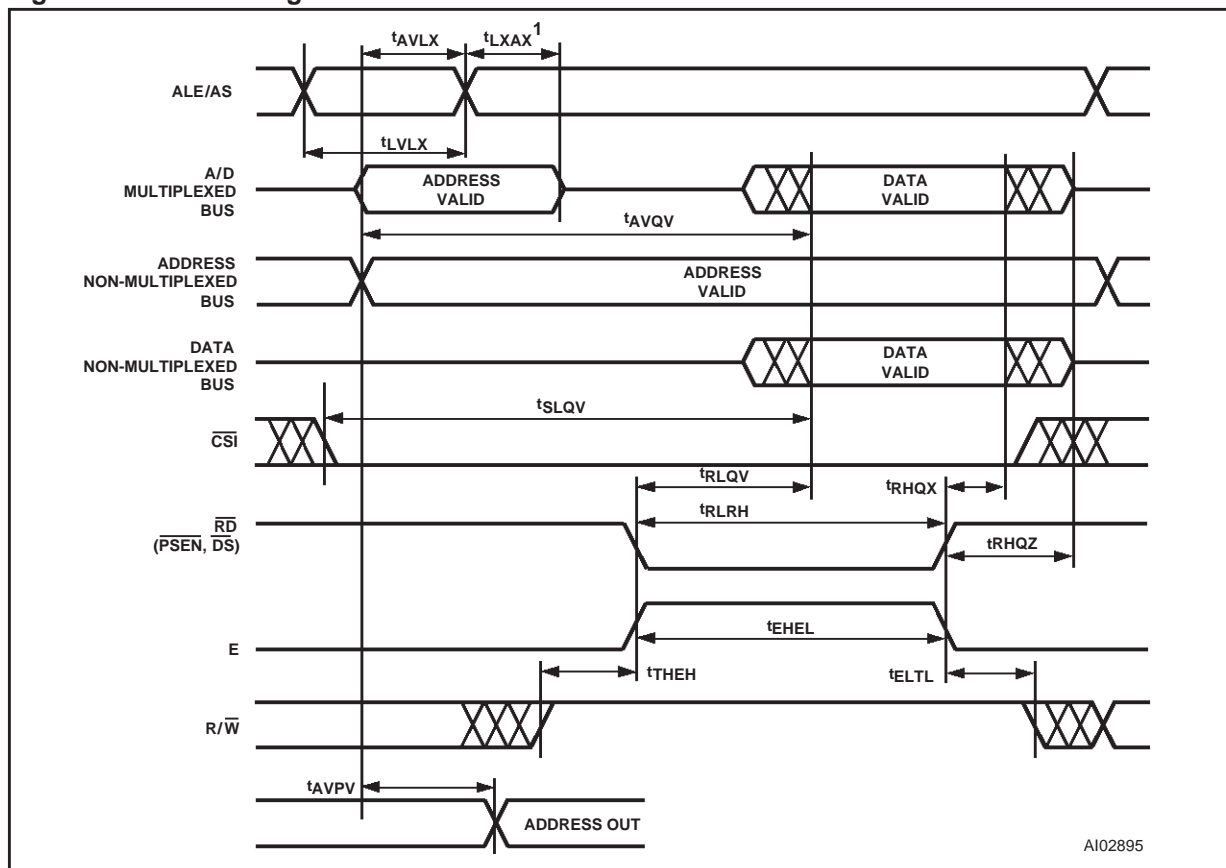
Figure 41. Read Timing
