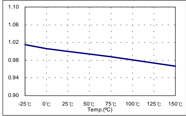
Figure 2. Stop Voltage
