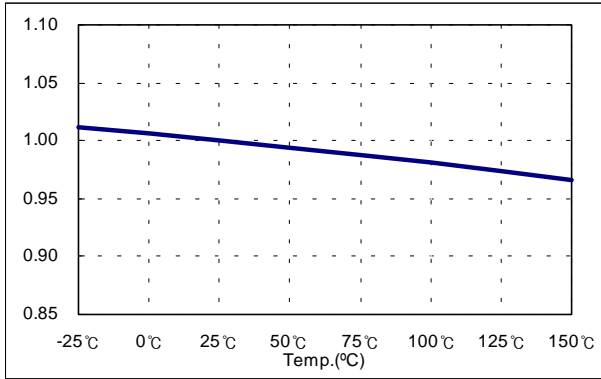
Figure 1. Start Voltage
