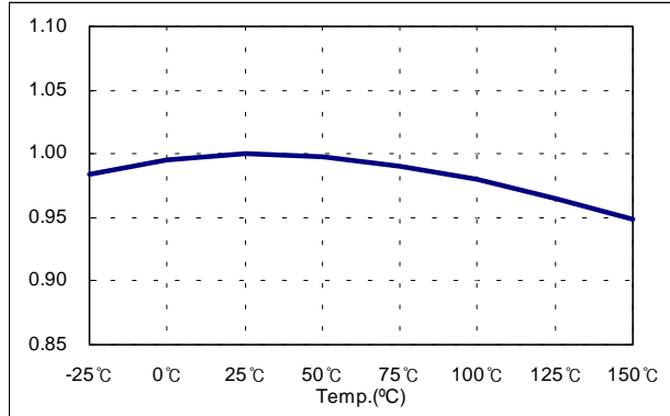
Figure 4. Operating Current
