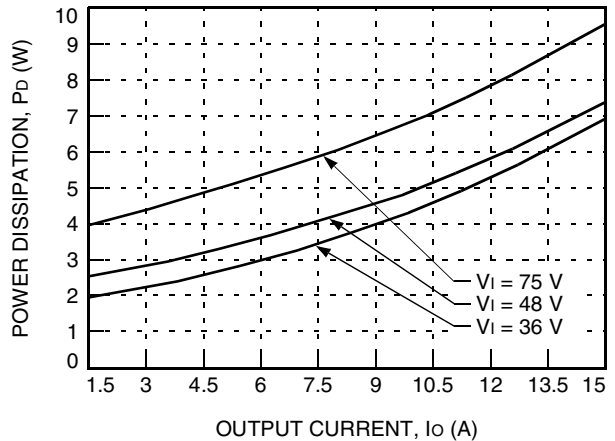
Figure 28. QHW075F1-Q Power Dissipation vs. Output Current at 25 °C
