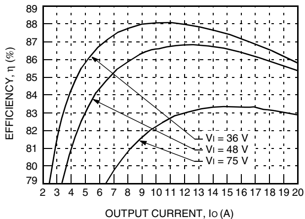
Figure 6. Typical QHW100F1-Q Converter Efficiency vs. Output Current at Room Temperature
