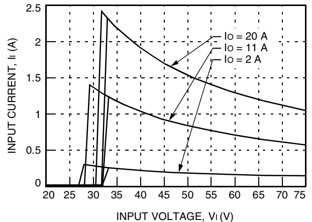
Figure 3. Typical QHW100F1-Q Input Characteristics at Room Temperature
