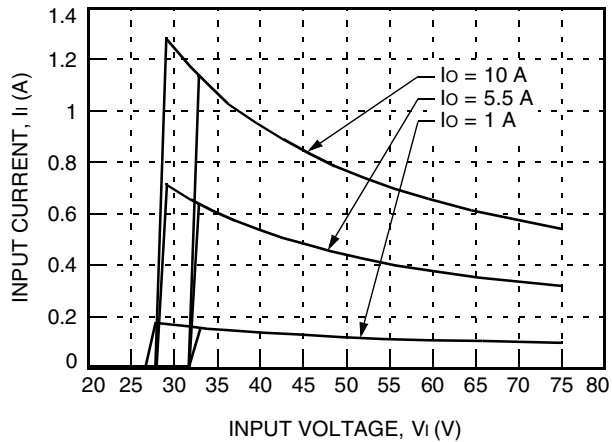
Figure 1. Typical QHW050F1-Q Input Characteristics at Room Temperature
