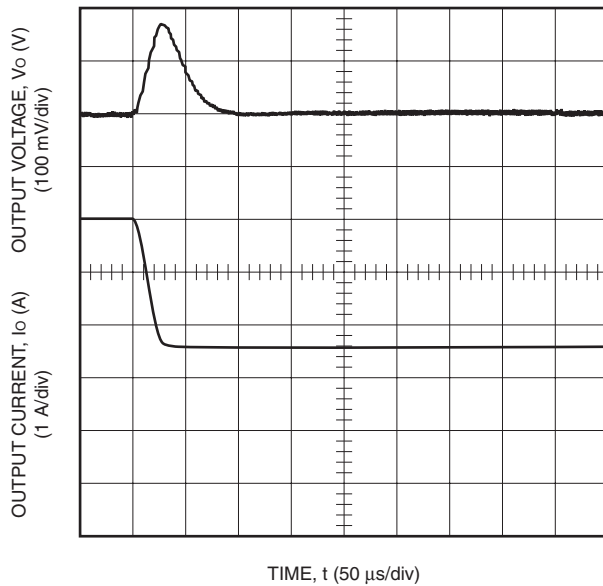
Figure 13. Typical QHW050F1-Q Transient Response to Step Decrease in Load from 50% to 25% of Full Load at Room Temperature and 48 Vdc Input. (Waveform Averaged to Eliminate Ripple Component.)
