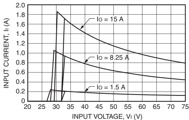
Figure 2. Typical QHW075F1-Q Input Characteristics at Room Temperature
