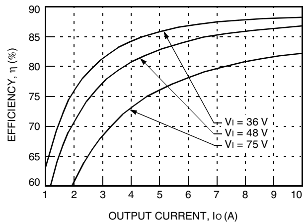
Figure 4. Typical QHW050F1-Q Converter Efficiency vs. Output Current at Room Temperature
