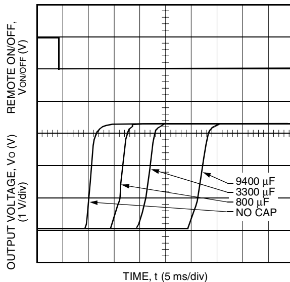
Figure 16. Typical Start-Up from Remote On/Off; I_o = I_{o, \max}
