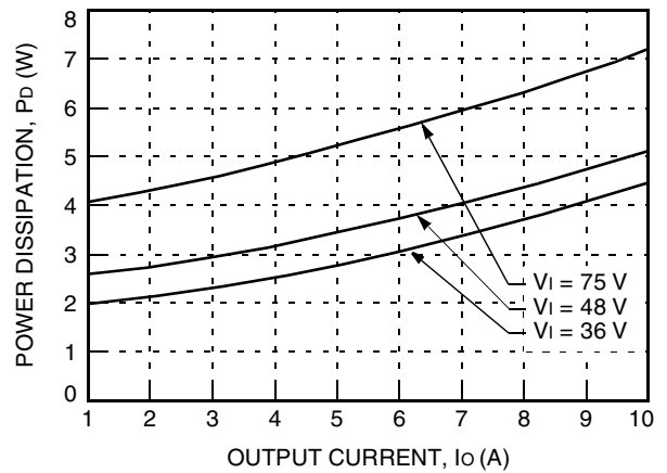
Figure 27. QHW050F1-Q Power Dissipation vs. Output Current at 25 °C
