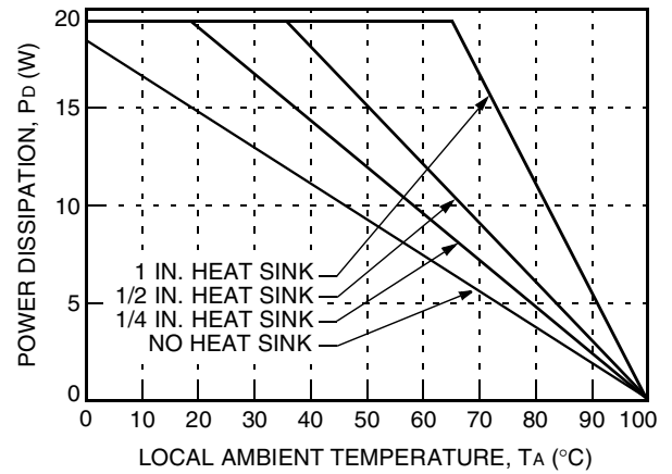
Figure 34. Heat Sink Power Derating Curves; 1.0 m/s (200 lfm); Transverse Orientation
