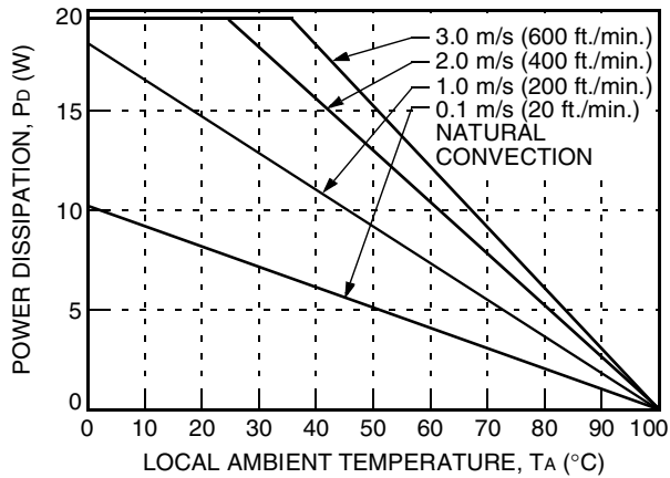
Figure 25. Forced Convection Power Derating with No Heat Sink; Transverse Orientation
