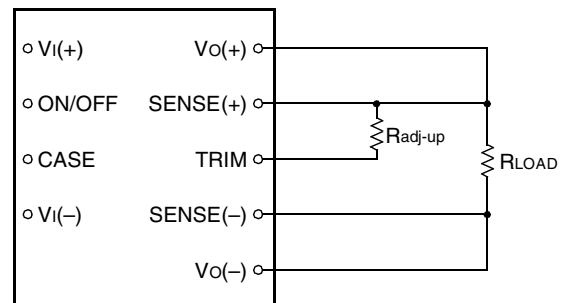
Figure 23. Circuit Configuration to Increase Output Voltage
