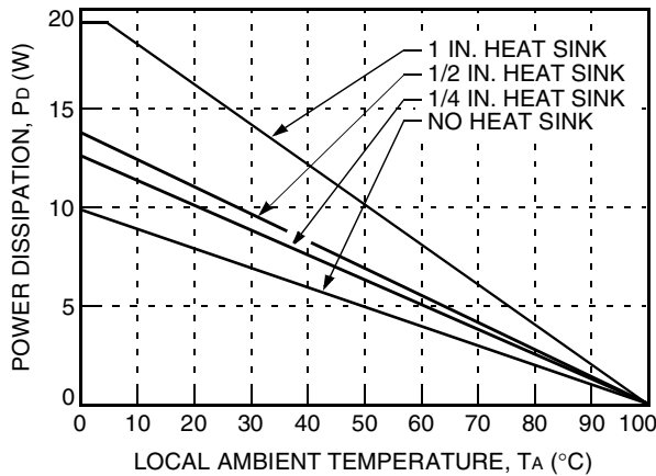
Figure 32. Heat Sink Power Derating Curves; Natural Convection; Transverse Orientation
