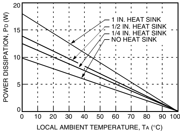
Figure 33. Heat Sink Power Derating Curves; Natural Convection; Longitudinal Orientation
