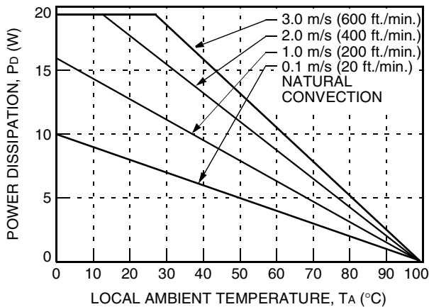
Figure 26. Forced Convection Power Derating with No Heat Sink; Longitudinal Orientation
