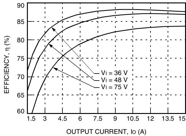
Figure 5. Typical QHW075F1-Q Converter Efficiency vs. Output Current at Room Temperature
