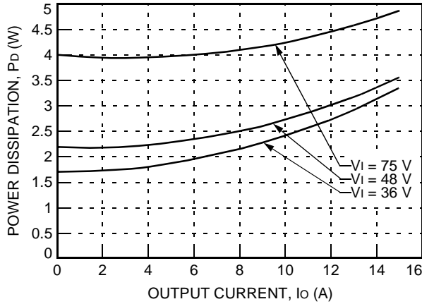
Figure 28. JAHW075Y Power Dissipation vs. Output Current at 25 °C
