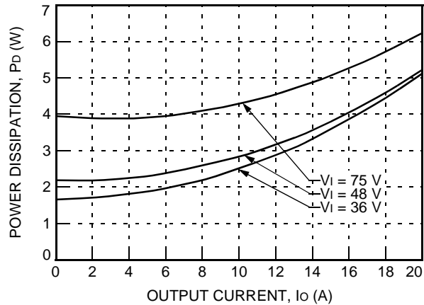
Figure 29. JAHW100Y Power Dissipation vs. Output Current at 25 °C
