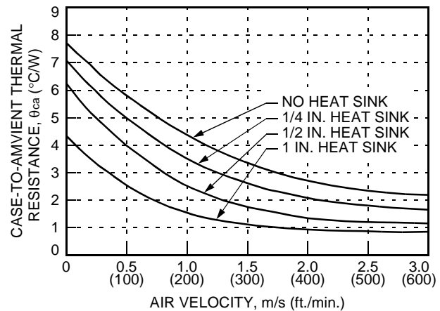
Figure 30. Case-to-Ambient Thermal Resistance Curves; Either Orientation
