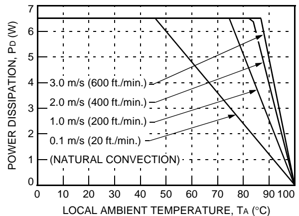
Figure 26. Forced Convection Power Derating with No Heat Sink; Either Orientation
