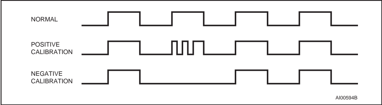
Figure 17. Calibration Waveform
