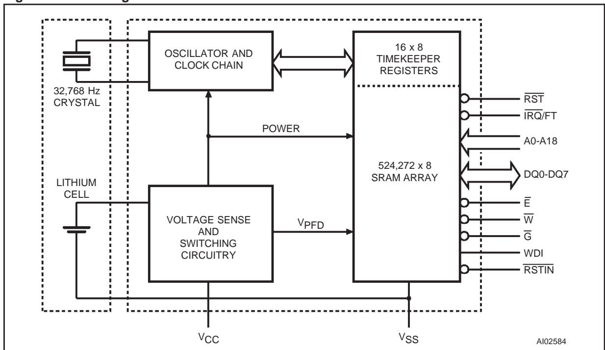
Figure 5. Block Diagram
