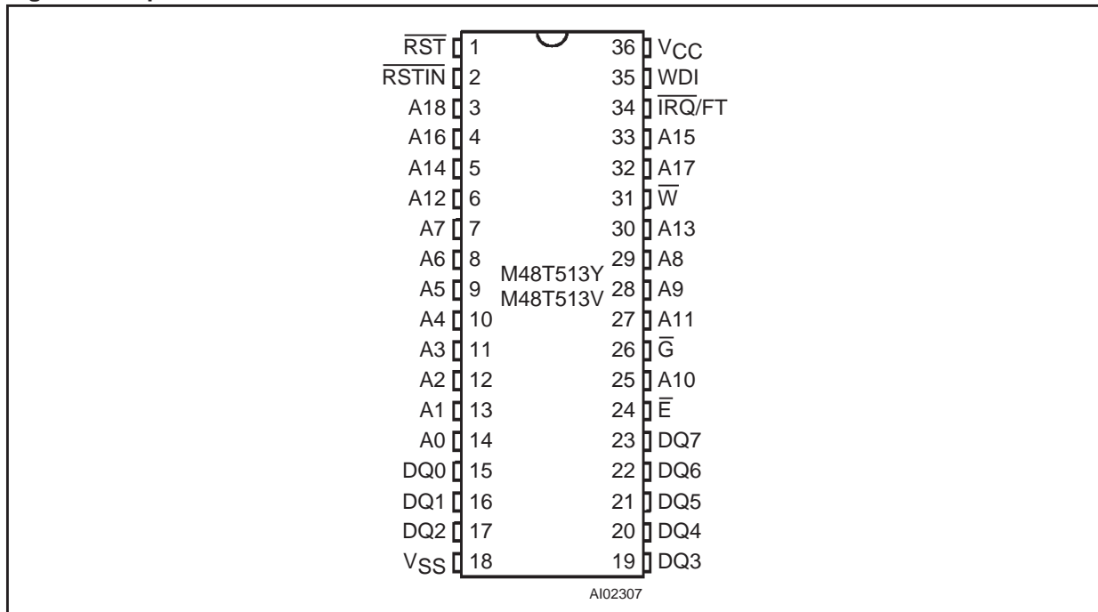
Figure 4. 36-pin Module Connections
