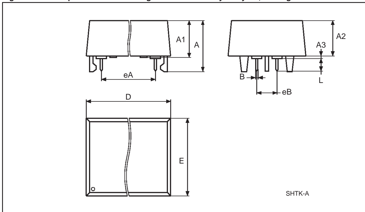
Figure 22. SH – 4-pin SNAPHAT Housing for 120mAh Battery &amp; Crystal, Package Outline
